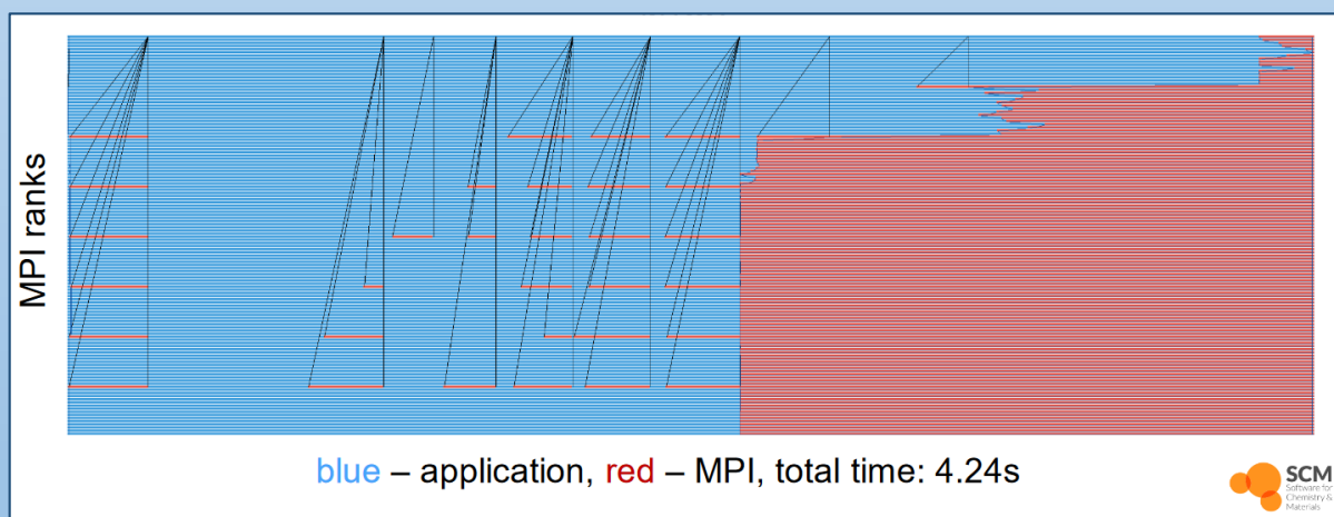
Original timeline of load balance for Hartree-Fock exchange, communication lines in black
